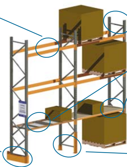
Shelving options with mesh decks or particle boards
